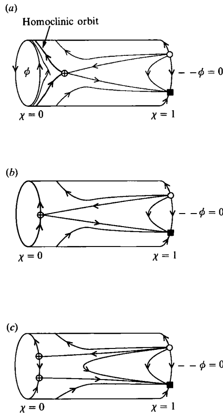
FIGURE 7. The cylindrical phase portraits corresponding to the averaged system of equations. (a) \frac{8}{3}\sqrt{2} > \beta > \beta_{\text{crit}} = 1/\sqrt{2} , (b) \beta = \beta_{\text{crit}} = 1/\sqrt{2} , (c) \beta < \beta_{\text{crit}} .
