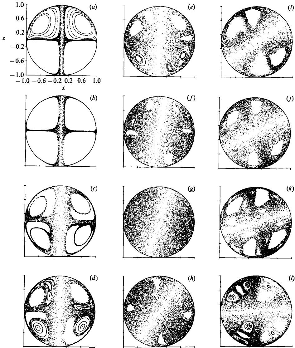
FIGURE 6. The effect of changing the orientation of the vorticity vector, |\omega| = 2.0 . (a-l) \theta = 0.001\pi, 0.002\pi, 0.0067\pi, 0.01\pi, 0.02\pi, 0.06\pi, 0.1\pi, 0.2\pi, 0.3\pi, 0.35\pi, 0.4\pi, 0.48\pi respectively.
